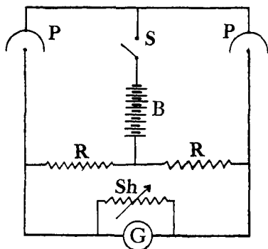
Fig. 2.—The photo-cell circuit: P, P, General Electric PJ14 photo-cells; S, switch; B, 90-volt battery; R, R, 100-000-ohm resistances; G, Leeds and Northrup wall galvanometer, resistance 1090 ohms, sensitivity 1133 meg-ohms, period 13.1 seconds; Sh, shunt box.
